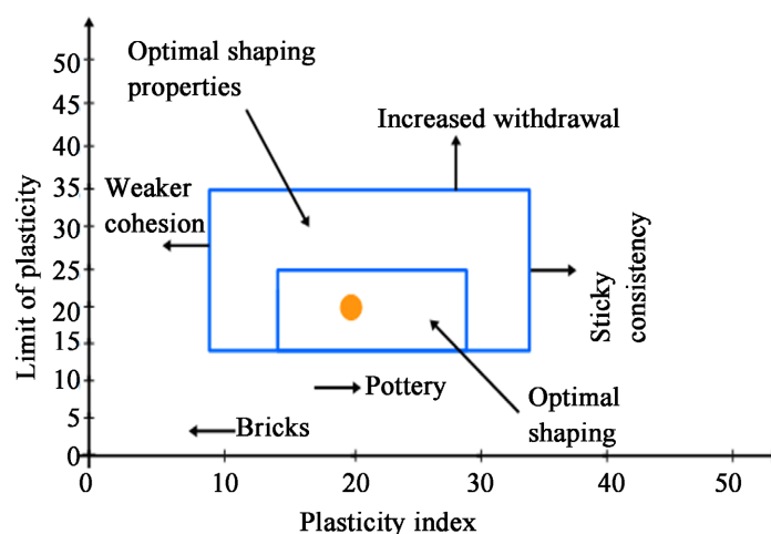
Figure 6. Positioning of the Loudima sample in the Bain and Higlyn workability map.
